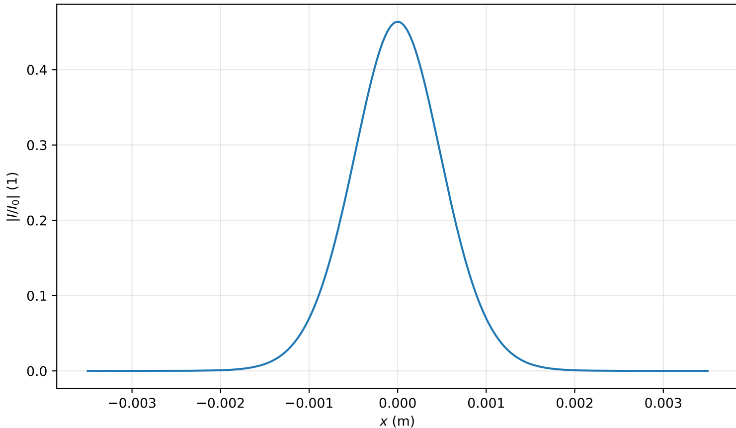
Intensity profile I(x, y = 0, z = 2.786m)/I_0 , P_{in}=0.3P_{cr} , artificial time
